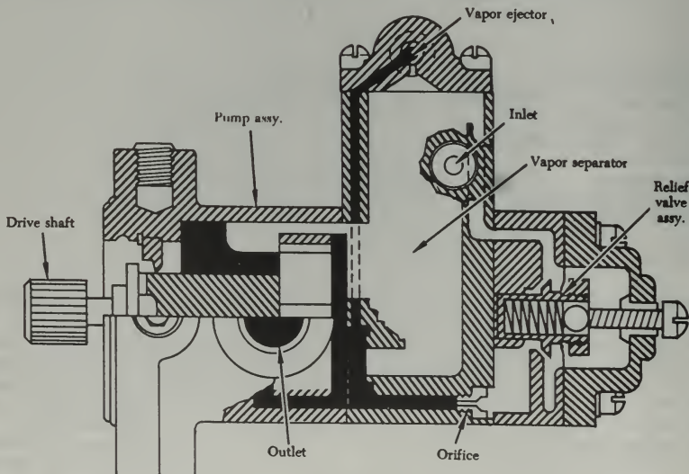
FIGURE 3-35. Fuel-injection pump.
